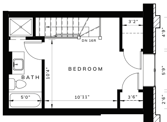
FLOOR 3
